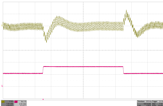
Figure 11: Regulated model output voltage response to step-change in load current with 200µF hold-up capacitor (50%-75%-50% of Iout(max), 115Vrms, 60Hz) Top: Vout (1V/div), Bottom: Iout (5A/div), Timebase: (100ms/div).
