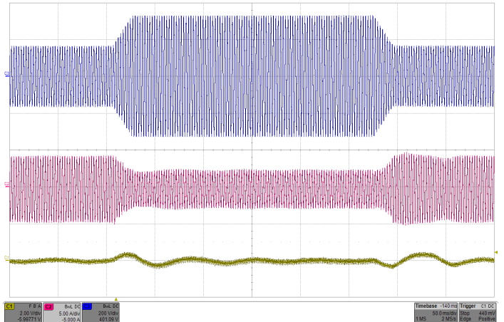
Figure 16: Input voltage transient response with 200µF hold-up capacitor at full load current (115Vrms-230Vrms-115Vrms, 400Hz), Top: Vin (200V/div), Mid: In (5A/div), Bottom: Vout (2V/div), Timebase: (50ms/div).
