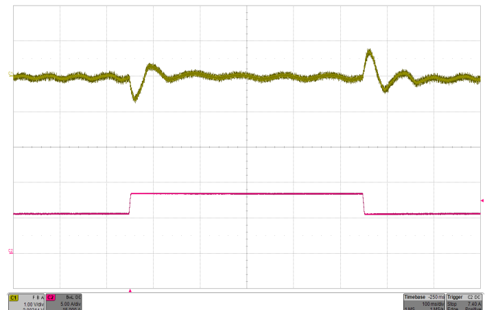
Figure 12: Regulated model output voltage response to step-change in load current with 200µF hold-up capacitor (50%-75%-50% of Iout(max), 115Vrms, 400Hz) Top: Vout (1V/div), Bottom: Iout (5A/div), Timebase: (100ms/div).
