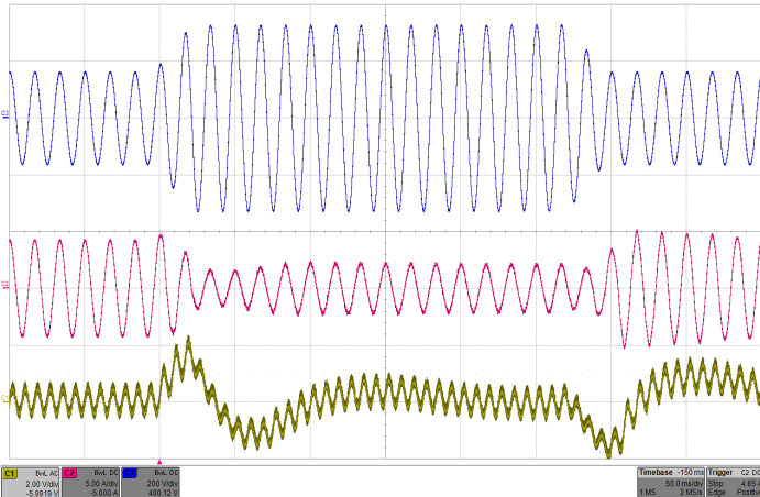
Figure 15: Input voltage transient response with 200µF hold-up capacitor at full load current (115Vrms-230Vrms-115Vrms, 60Hz), Top: Vin (200V/div), Mid: In (5A/div), Bottom: Vout (2V/div), Timebase: (50ms/div).
