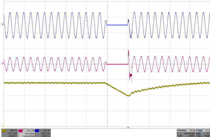
Figure 9: Line drop out with 400µF hold-up capacitor at full load current (115Vrms, 60Hz) Top: Vin (200V/div), Mid: Iin (10A/div), Bottom: Vout (10V/div), Timebase: (50ms/div).
